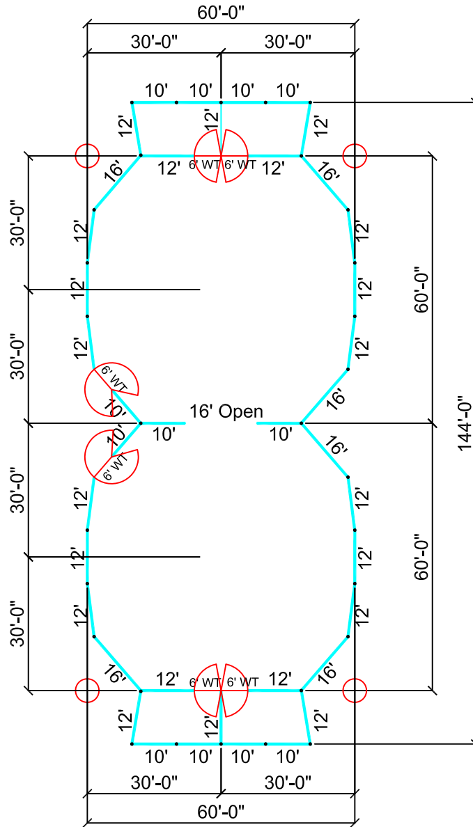
60FT. Sorting Arena (12 FT. PANELS)
